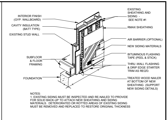
RMAX SHEATHING IN A RESIDING APPLICATION
