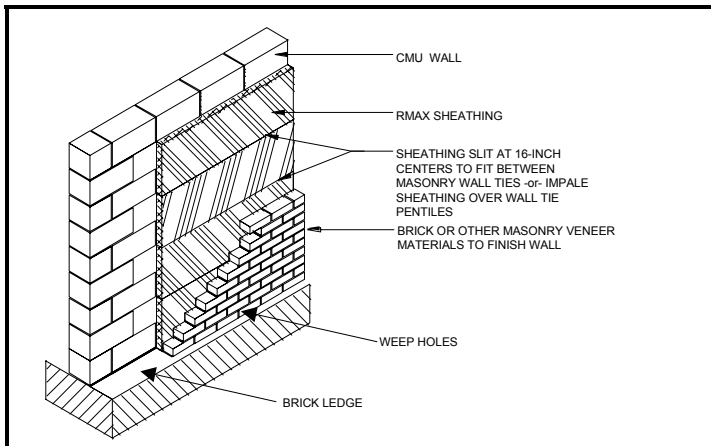
RMAX SHEATHING APPLIED OVER CONCRETE MASONRY AND BRICK VENEER WALLS.
