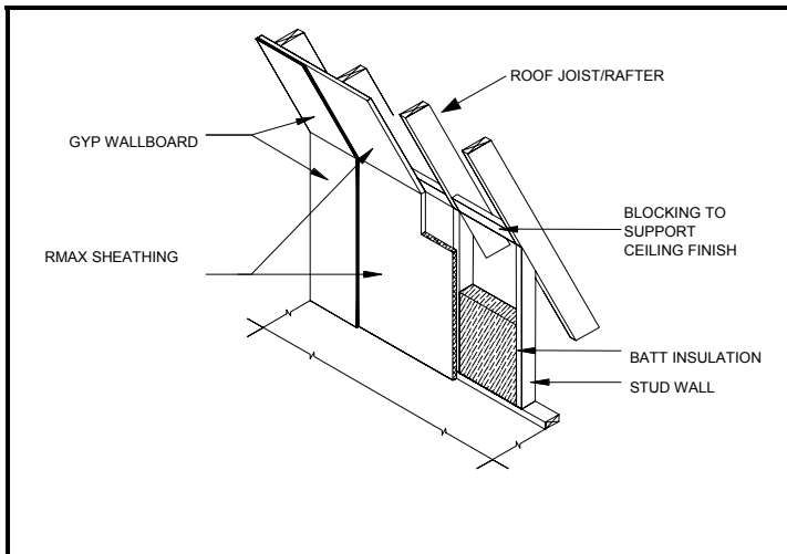
INTERIOR USE OF SHEATHING ON STUD WALL AND ROOF RAFTERS
