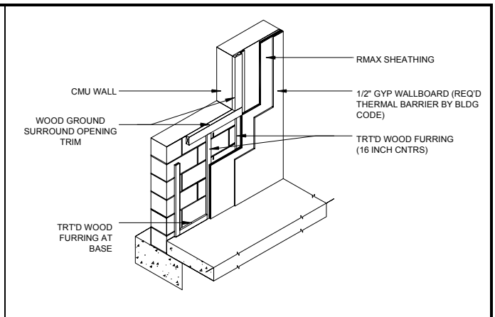
RMAX SHEATHING APPLIED TO INTERIOR SIDE OF CONCRETE MASONRY WALLS.
